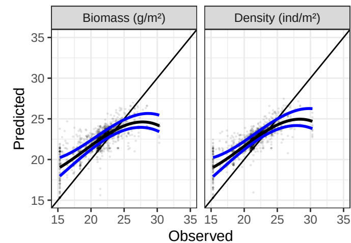
% Intolerant Taxa
