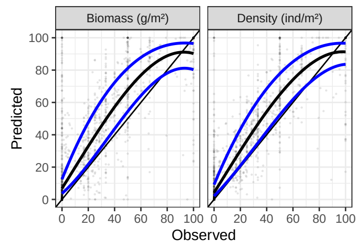
% Intolerant Taxa
